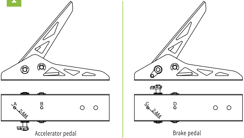
Figure 1: Take out the brake pedal and accelerator pedal, and check the mounting holes.
