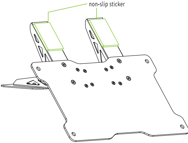
Figure 5: Paste anti-slip pads on the bottom plate of the reversible pedal, and paste one piece each on the accelerator pedal and brake pedal to complete the assembly.
