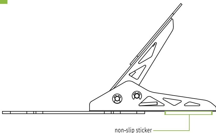
Figure 4: Take out the non-slip sticker, tear off the film and paste it on the suspended position where the pedal and the bottom plate do not overlap.
