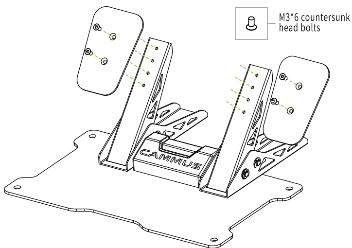
Figure 3: The pedals can be placed where the user is most comfortable with, then take 4 M3*6 countersunk head bolts to align and attach them in place.
