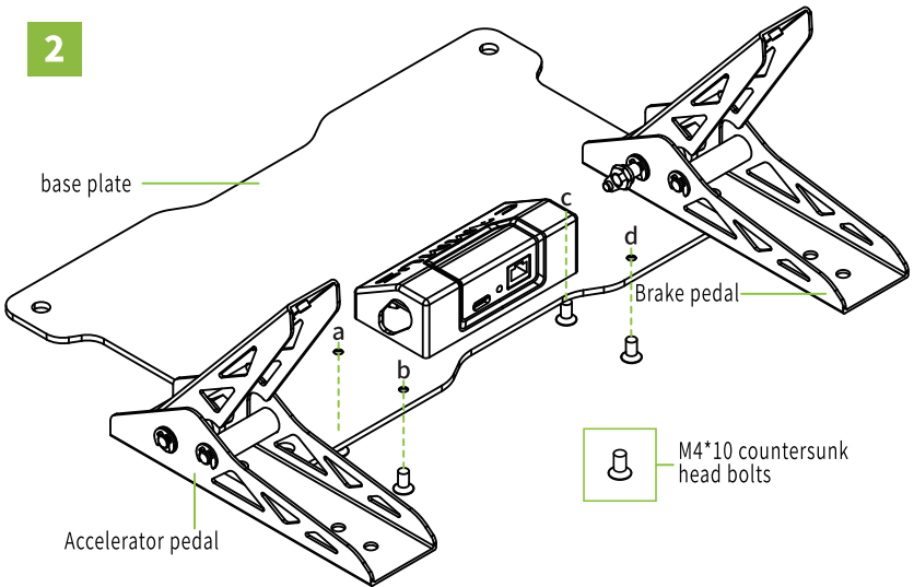
Figure 2: Place the pedal on the base plate, align the protruding shaft with the opening of the base plate box and push it into the opening. Use M4*10 countersunk head bolts to lock from the bottom up, align the holes in the order of A-a, B-b, C-c, D-d to lock.
